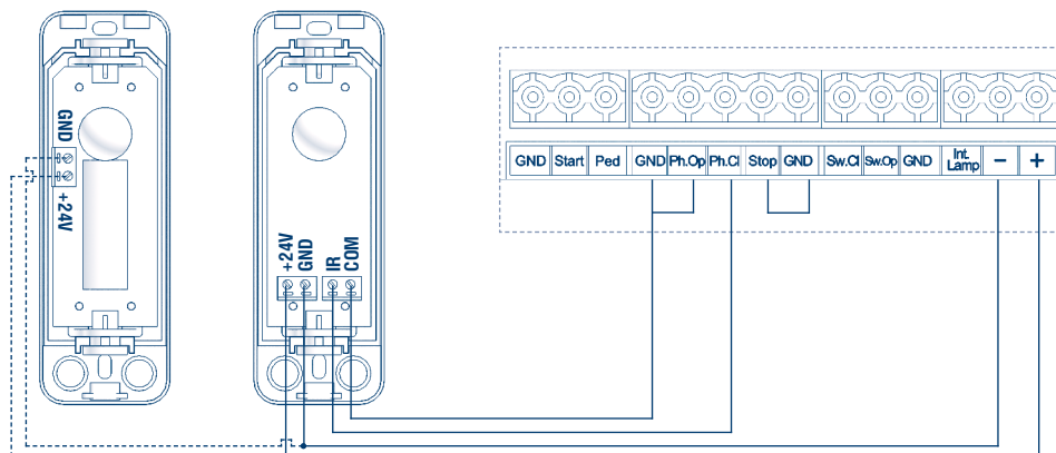
Рис./Fig. 16. SWING-3000/4000/5000(PRO), ARM-320PRO
