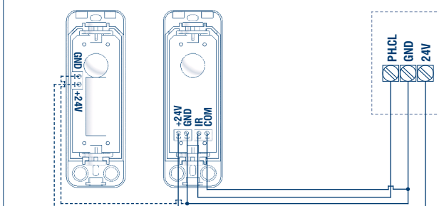
Рис./Fig. 19. SECTIONAL-800PRO/1000PRO/1200/1200PRO, FAST-800PRO
