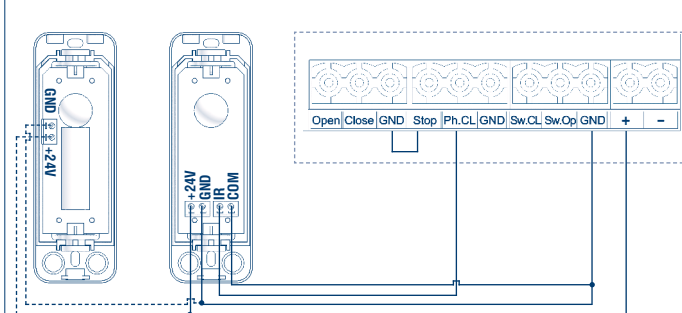
Рис./Fig. 19. SECTIONAL-800PRO/1000PRO/1200/1200PRO, FAST-800PRO
