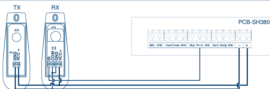
Рис./Fig. 12. SECTIONAL-800PRO/1000PRO/1200/1200PRO, FAST-800PRO
